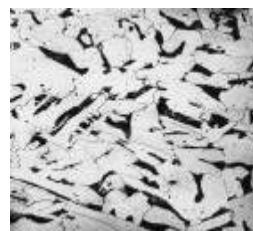
Fig. 1. Steel structure St3ps, × 500
